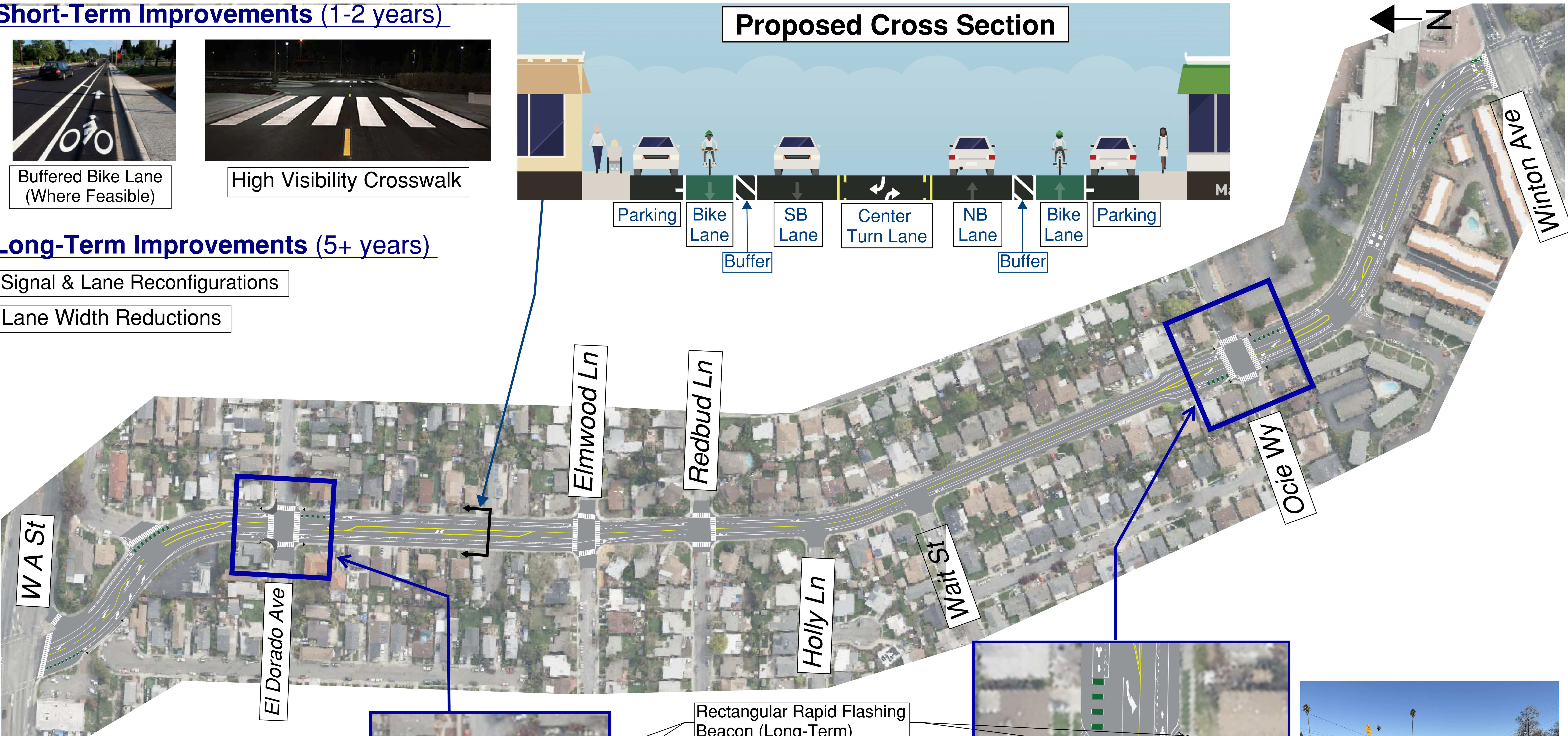
Curb Extension (Long-Term)
