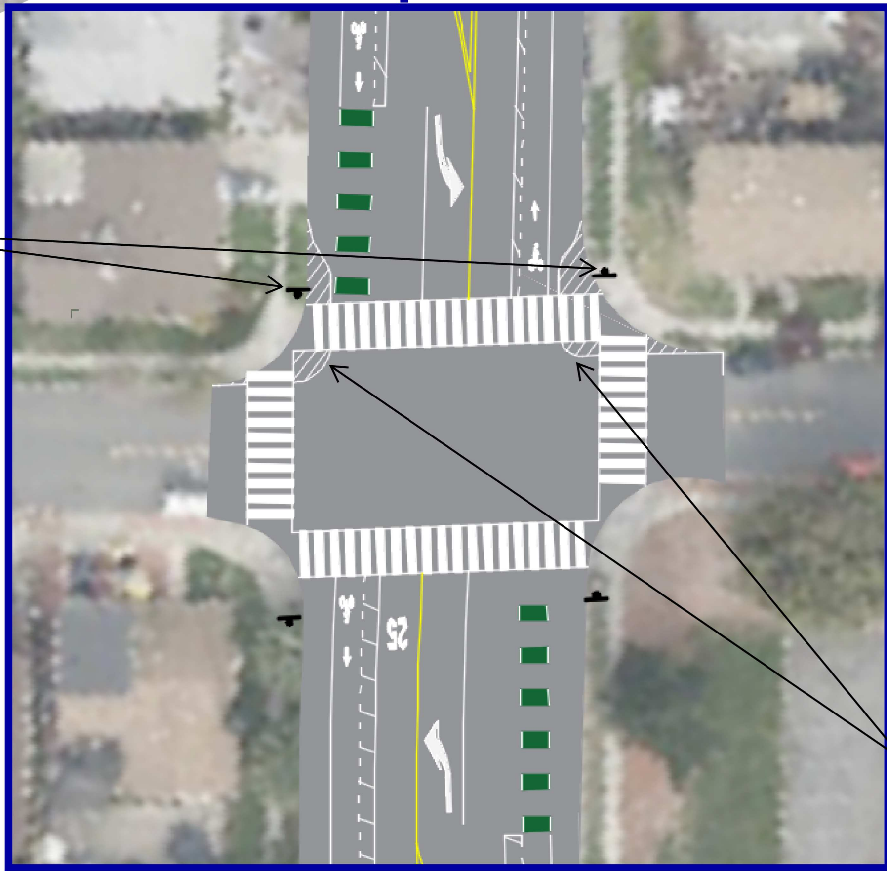
Painted Bulb-Out (Short-Term)
