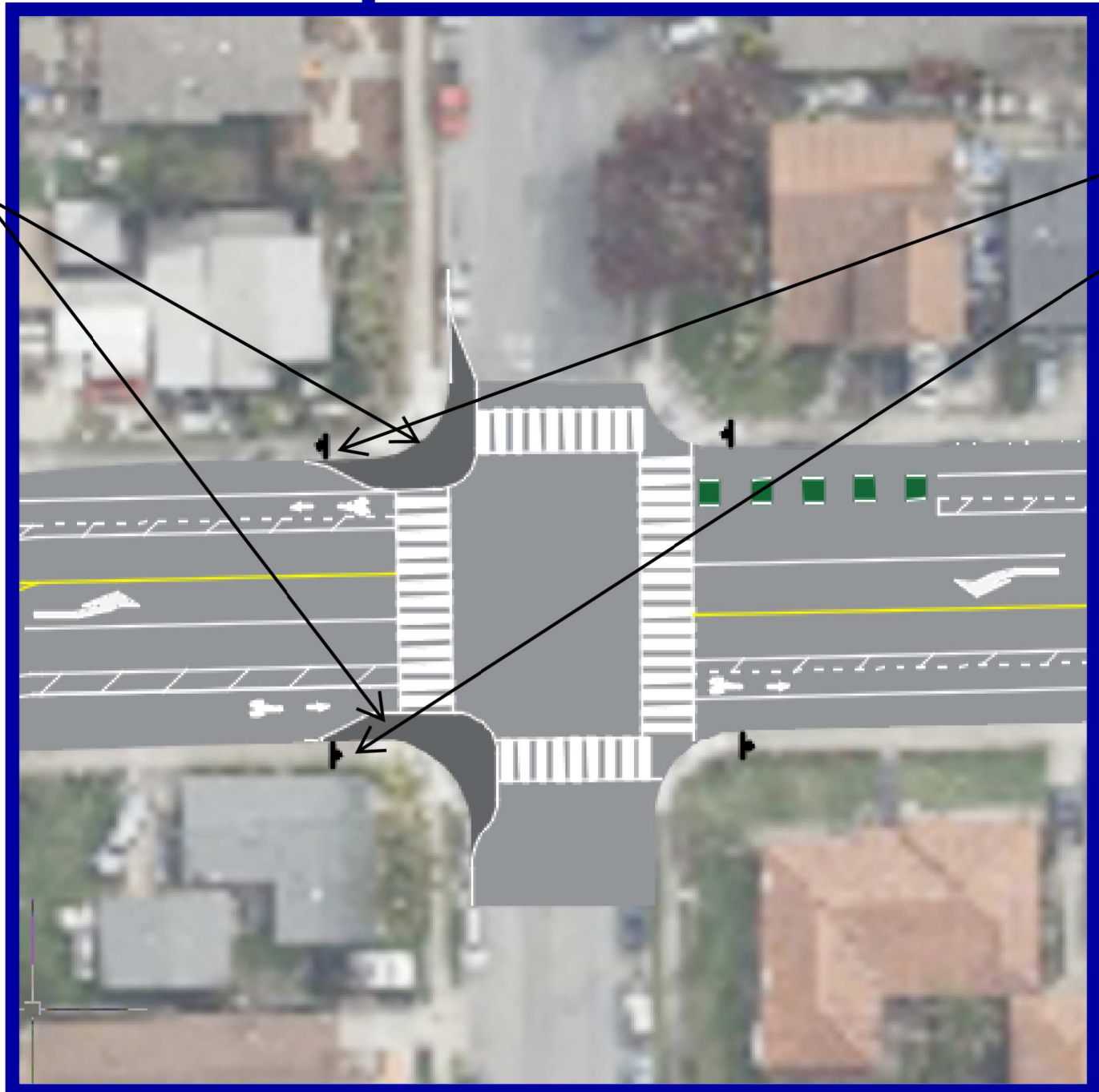
Curb Extension (Long-Term)
