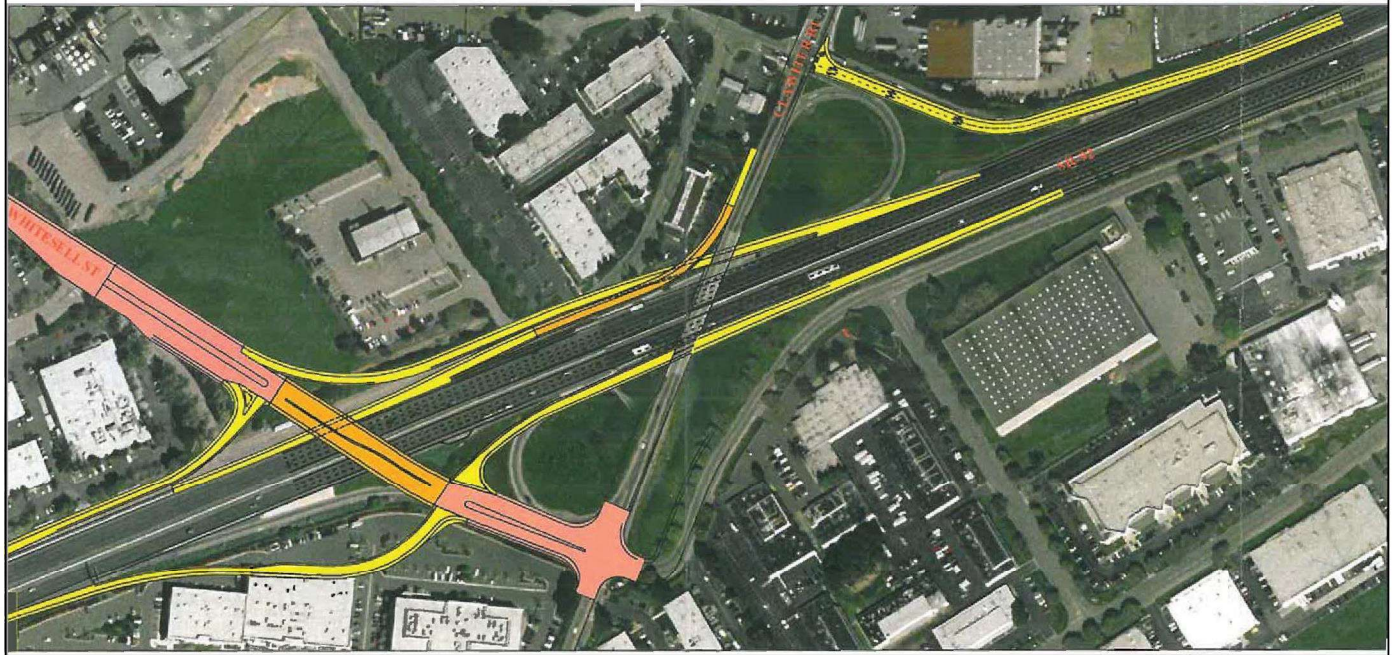
PROPOSED IMPROVEMENTS
